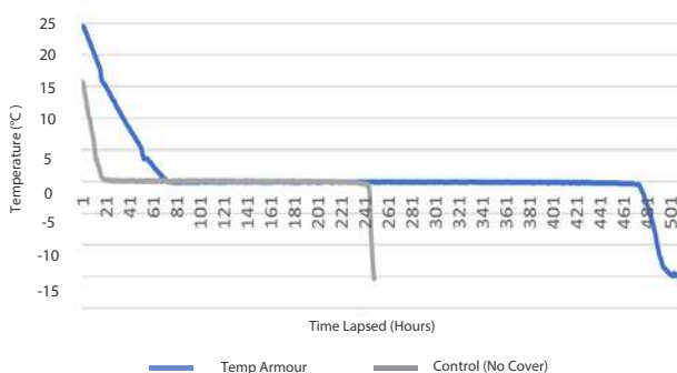
Freeze Time Comparative Data
